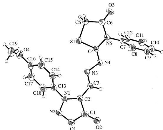
Figure 1. Crystal structure of compound 5c .
