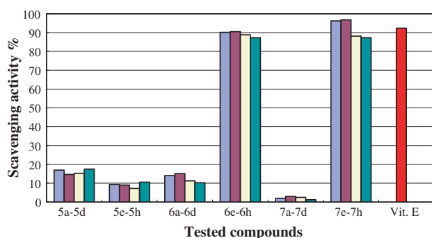
Figure 4. Scavenging activity of compounds 5a–7h (0.1 mM) incubated 30 min with DPPH at 0.1 mM concentration.
