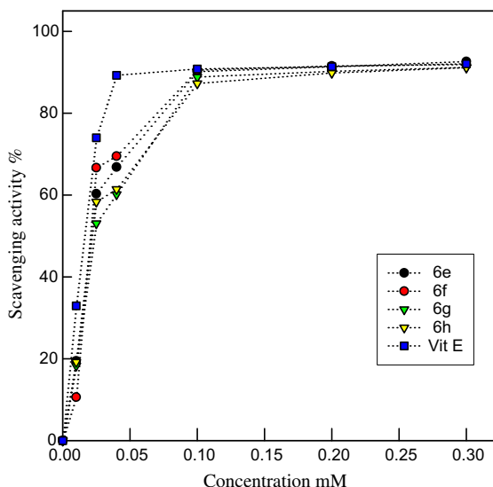
Figure 5. Scavenging activity of compounds 6e–h on DPPH radical.
