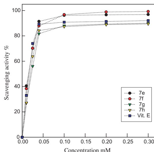
Figure 6. Scavenging activity of compounds 7e–h on DPPH radical.
