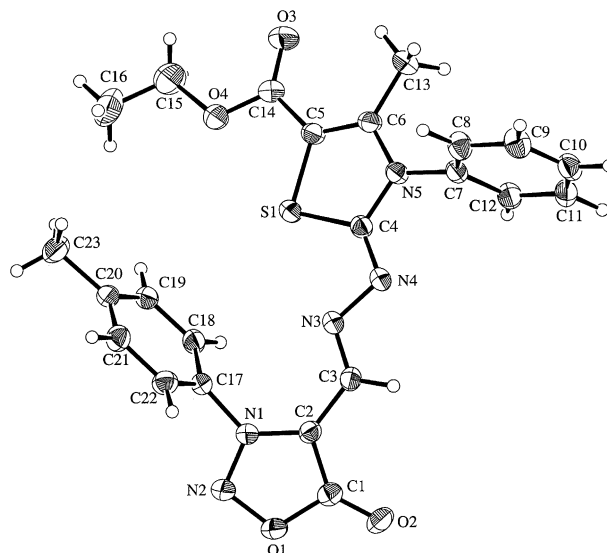
Figure 2. Crystal structure of compound 6b .
