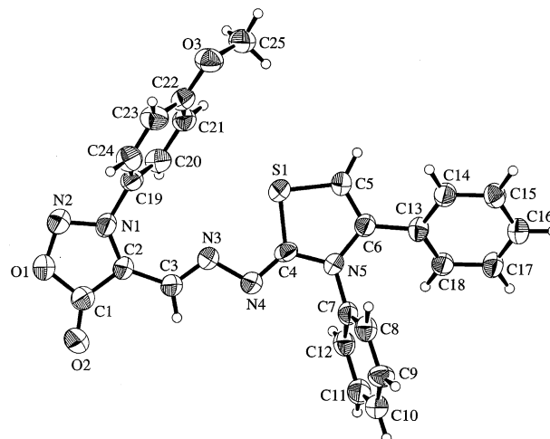
Figure 3. Crystal structure of compound 7c .
